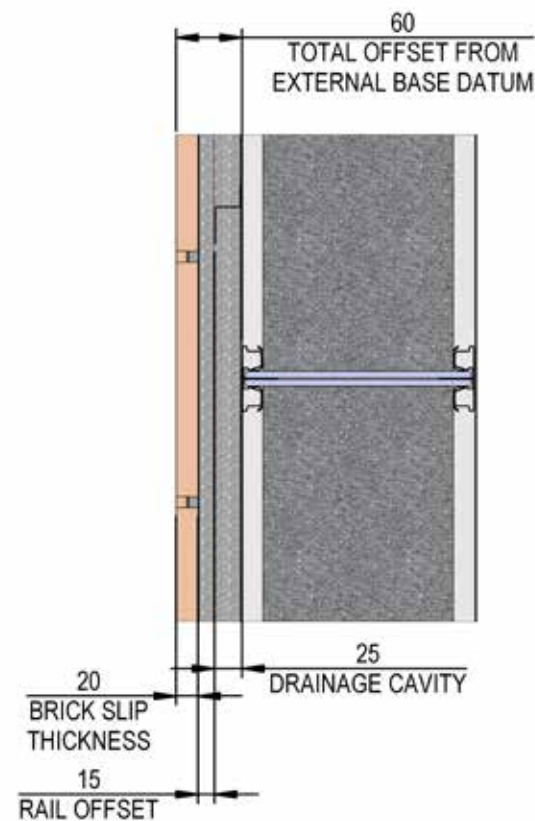
hup! walls with brick slips rails
