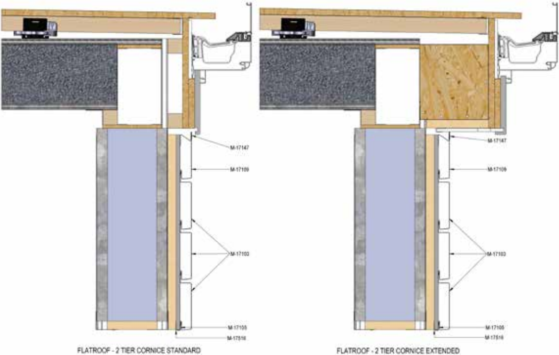
Flat Roof 2 tier with steel facade
